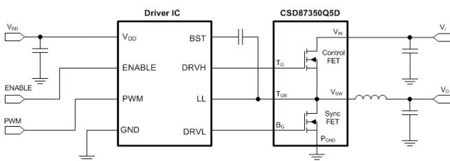
TYPICAL CIRCUIT
