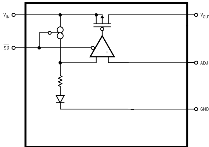
Figure 4. LP3875-ADJ
