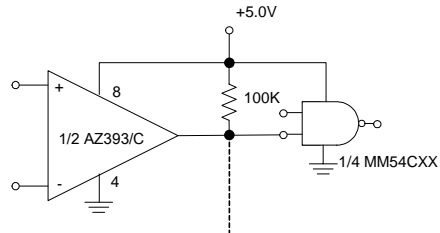
Figure 10. Driving CMOS/TTL
