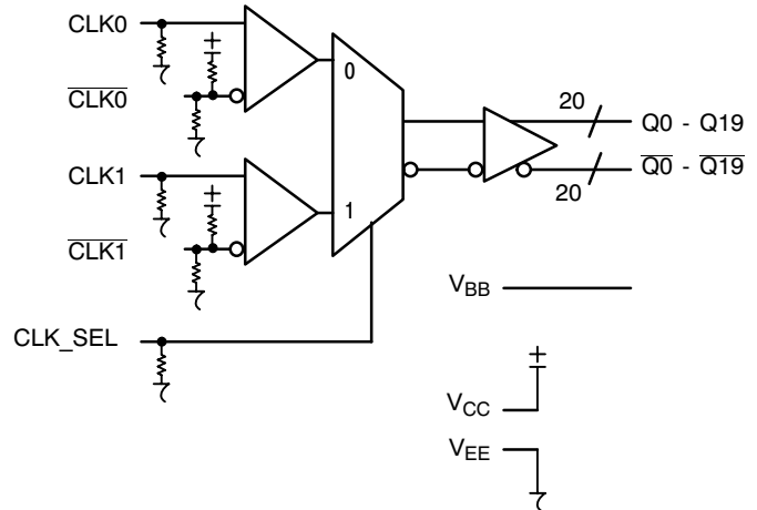
Figure 3. Logic Diagram
