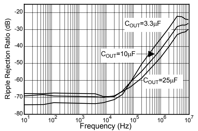
Fig. 6 AIC1117 (ADJ) Ripple Rejection Ratio (dB)
