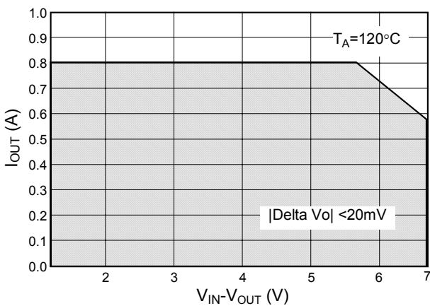
Fig. 5 AIC1117 (ADJ) Maximum Output Current vs. V_{IN}-V_{OUT}
